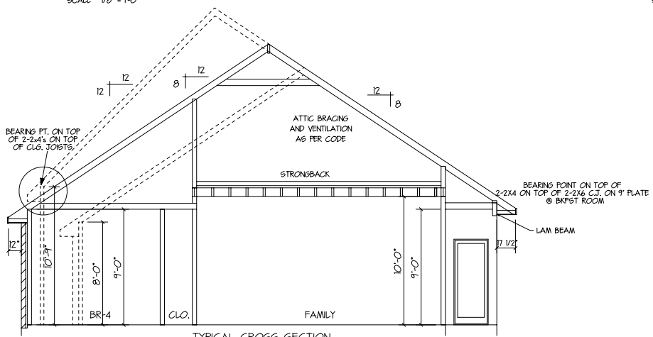
TYPICAL CROSS SECTION SCALE 1/4" = 1'-0"
