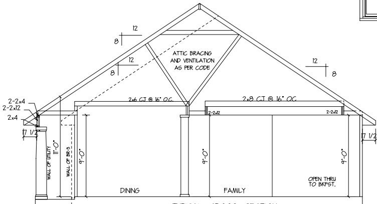
TYPICAL CROSS SECTION SCALE 1/4" = 1'-0"
